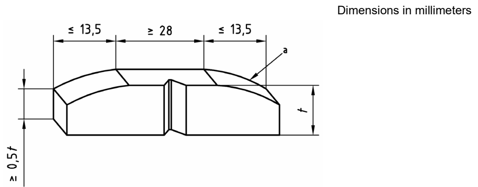
Figure D.12—Charpy Specimen Dimensions
